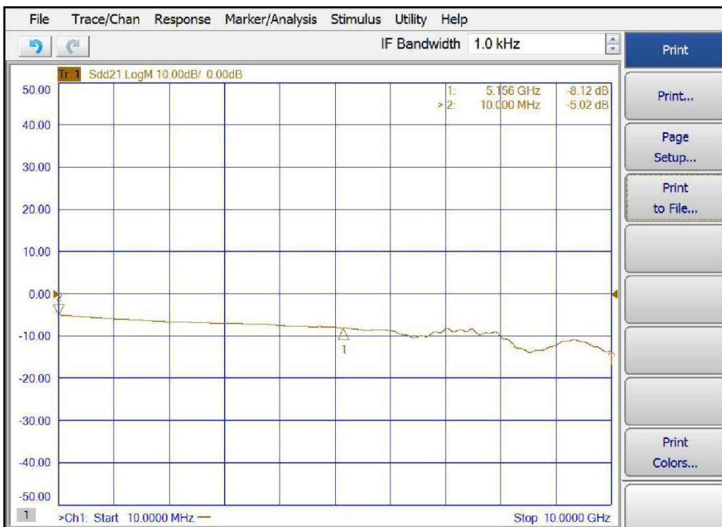
SDD21-5dB (Transmit Insertion Loss)
